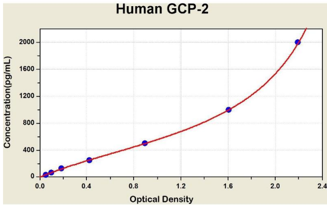
Image 1. Diagramm of the ELISA kit to detect Human GCP-2 with the optical density on the x-axis and the concentration on the y-axis.
