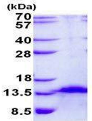
15% SDS-PAGE (3ug)
