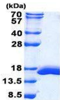
15% SDS-PAGE (3ug)
