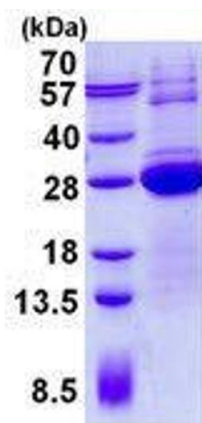
15% SDS-PAGE (3ug)
