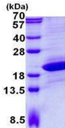
15% SDS-PAGE (3ug)
