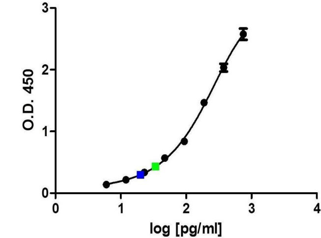
ELISA Image 1.
