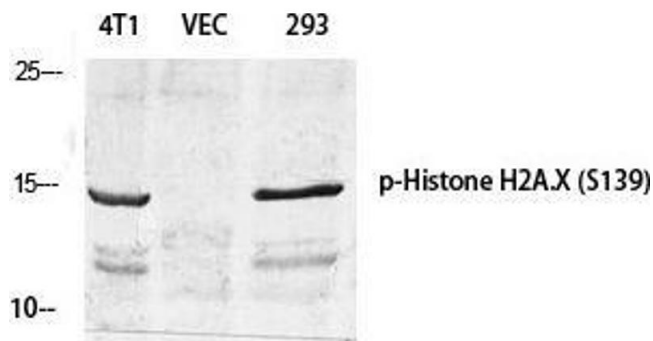
Image 2. Western Blot (WB) analysis of specific cells using Phospho-Histone H2A.X (S139) Polyclonal Antibody.
