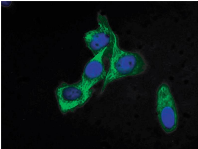
Image 1. Human mammary gland carcinoma cell line HCC38 was stained with Mouse Anti-Cytokeratin 18-FITC followed by DAPI.
