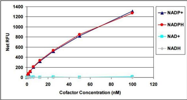
Image 2. NADP+ Standard Curve and Specificity of Assay for NADP+ and NADPH. NADP+ , NADPH, NAD+ , and NADH, were tested in the NADP+ /NADPH Assay Kit.
