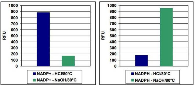
Image 3. NADP+ /NADPH Detection. NADP+ and NADPH were both tested at 100 nM with the extraction procedure. NADP+ or NADPH were incubated for 60 minutes at 80°C with 0.1N HCl or 0.1N NaOH.
