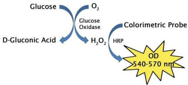
Image 1. Glucose assay principle.
