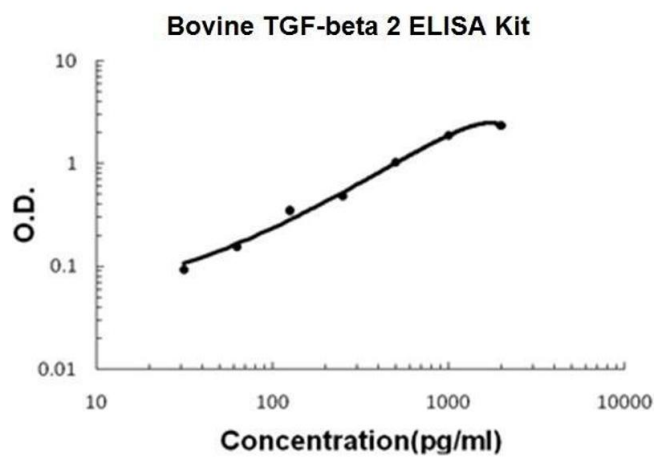
Image 1. Bovine TGF-beta 2 PicoKine ELISA Kit standard curve
