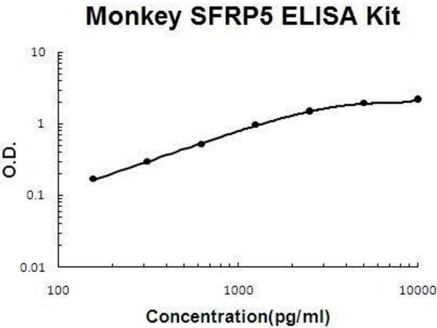
ELISA Image 1. Monkey Primate SFRP5 PicoKine ELISA Kit standard curve
