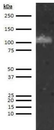
Figure 1: Western Blot
