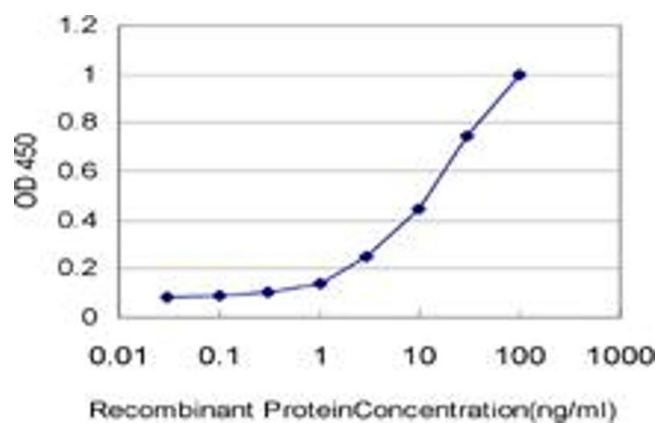
Image 2. Detection limit for recombinant GST tagged CD40LG is approximately 0.3ng/ml as a capture antibody.
