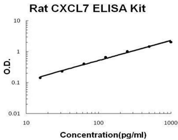
ELISA Image 1. Rat CXCL7 PicoKine ELISA Kit standard curve
