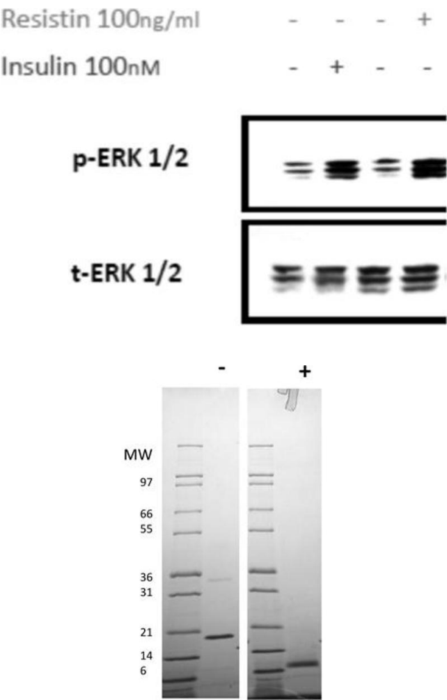
SDS-PAGE Image 1. SDS-PAGE of Human Resistin Dimer Recombinant Protein Bioactivity of Human Resistin Dimer Recombinant Protein. 100ng/mL of SBT recombinant Human Resistin or 100 nM Insulin (+ control) was added to differentiated SH-SY5Y cells. After 10 minutes MAPK activity was measured by western blotting whole cell lysates for P-Erk and Total Erk. The figure shows that Human Resistin is able to active MAPK signaling at 100ng/mL.
