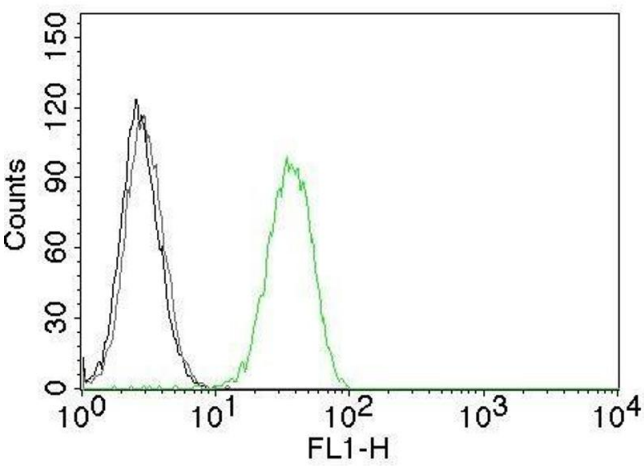
Flow Cytometry Image 1. Flow Cytometry of human CD31 on Jurkat cells. Black: cells alone; Grey: Isotype Control; Green: CF488-labeled CD31 Monoclonal Antibody (C31.7).
