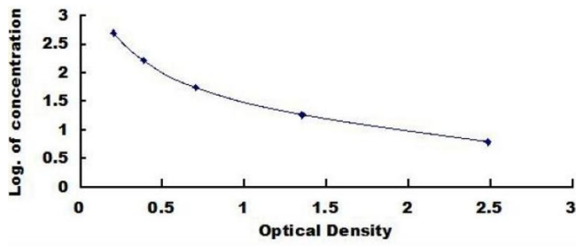
Typical Standard Curve for CP, Porcine ELISA.
