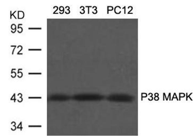
Western Blotting Image 1. Western blot analysis of extracts from 293, 3T3 and PC12 cells using P38 MAPK(Ab-180/182) Antibody.
