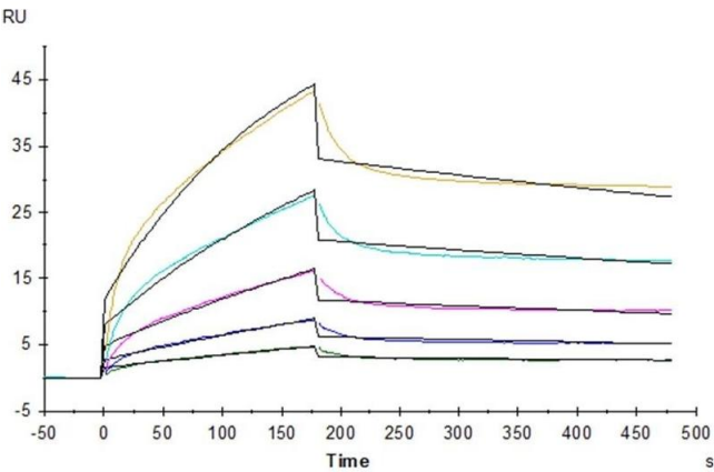
Image 1. Human ICOS, hFc Tag captured on CM5 Chip via Protein A can bind Cynomolgus B7-H2, His Tag with an affinity constant of 5.42 nM as determined in SPR assay (Biacore T200).
