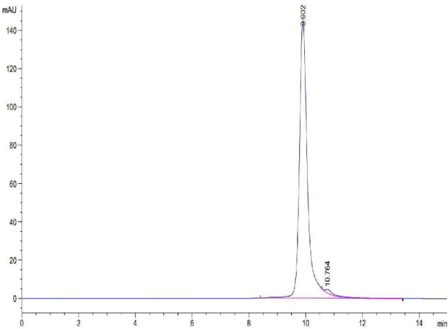
Image 2. The purity of Human FOLR4/Juno is greater than 95 % as determined by SEC-HPLC.
