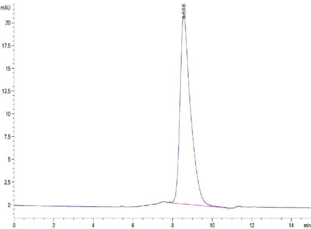
Image 2. The purity of Mouse GPVI is greater than 95 % as determined by SEC-HPLC.
