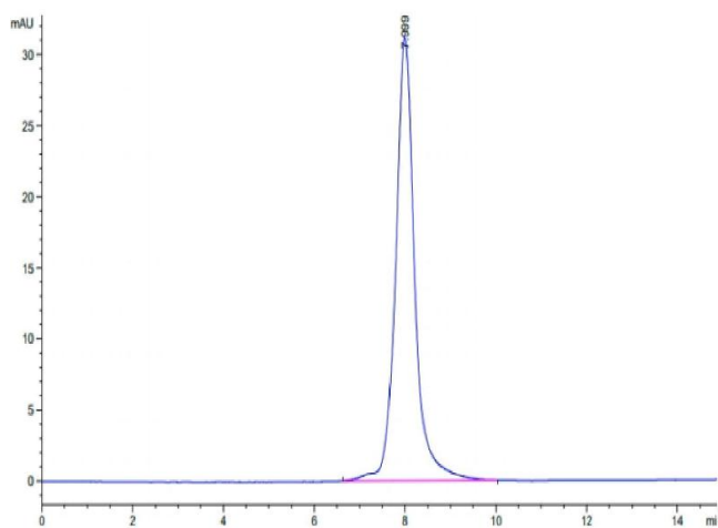
Image 2. The purity of Cynomolgus LILRB1 is greater than 95 % as determined by SEC-HPLC.
