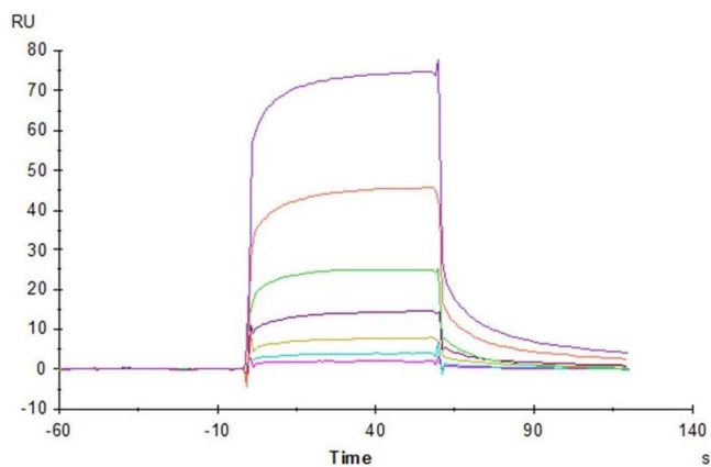
Image 1. Anti-LILRB1 Antibody, hFc Tag captured on CM5 Chip via Protein A can bind Cynomolgus LILRB1, His Tag with an affinity constant of 5.86 \mu M as determined in SPR assay (Biacore T200).
