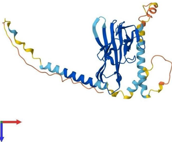
Protein Structure Image 1. AlphaFold protein structure prediction of Human Recombinant TNFSF11 Protein, UniprotID O14788
