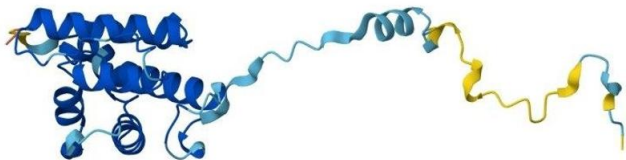
Image 1. AlphaFold protein structure prediction of Mouse Recombinant TagIn3 Protein, UniprotID Q9R1Q8
