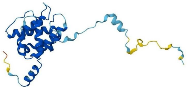
Image 2. AlphaFold protein structure prediction of Mouse Recombinant TagIn3 Protein, UniprotID Q9R1Q8
