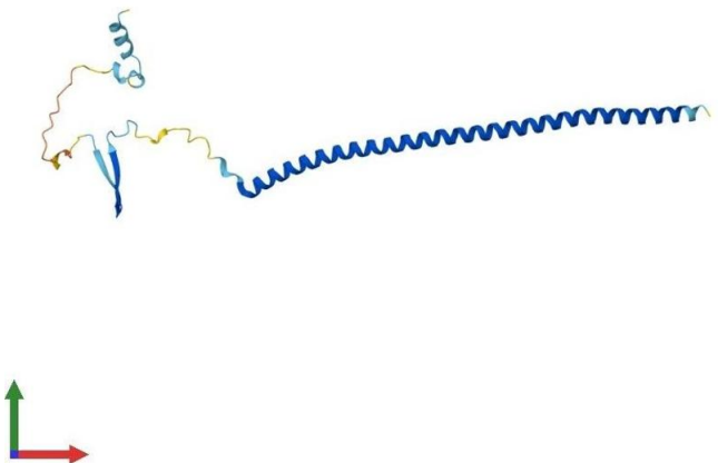
Image 2. AlphaFold protein structure prediction of Mouse Recombinant Stmn4 Protein, UniprotID P63042
